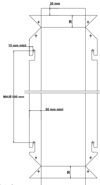
Figure 2 – Cassette (principe)
