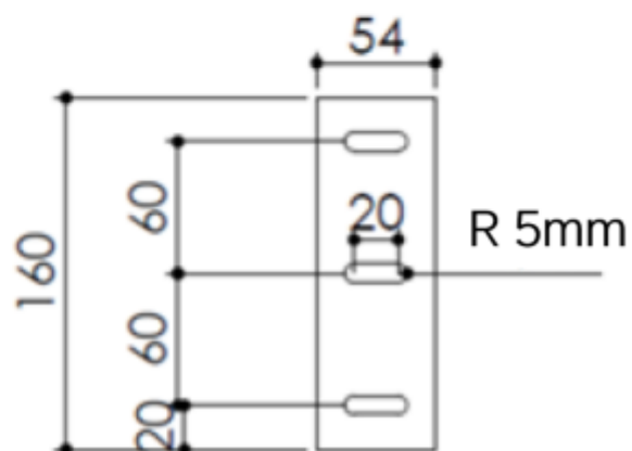
Figure A2a – Etrier (Tableau A2)
