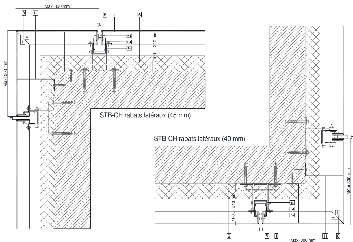
Figure 10 – Angle sortant – Coupe horizontale
